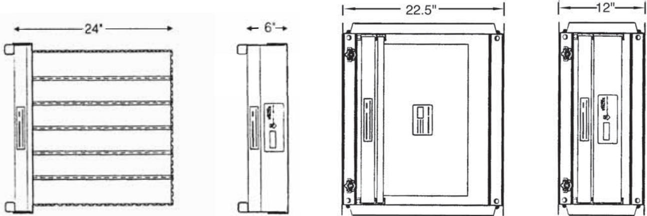
Astr Holding Frame with PrecisionPak and Pre Pleat 40
